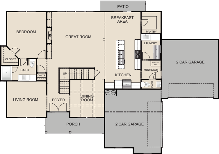
1st Floor
