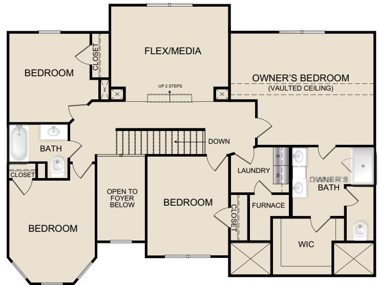
2nd Floor
